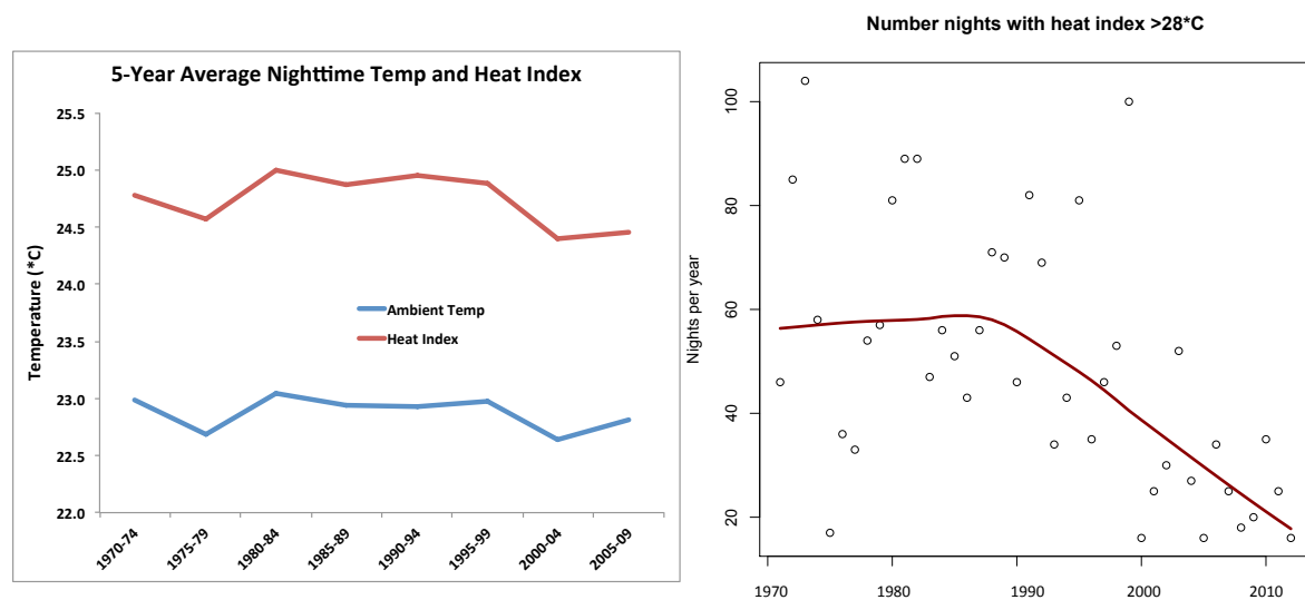
Figure 7: Trends in average nighttime temperatures and average heat values between 1970-2011 (left figure) and trends in the number of very hot nights where the heat index exceeds 28°C over the same period (right figure). The declining trend in very hot nights is significant at the 95th percentile and begins roughly around 1995. See accompanying text for possible explanation of the declining trend in very hot nights.
